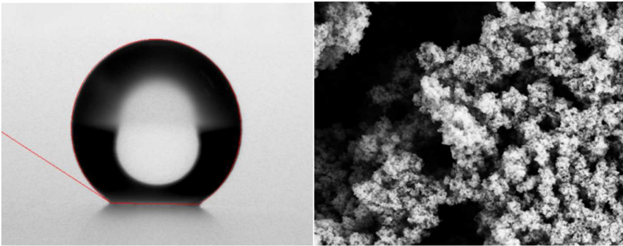
Water droplet on Lotus WC2 coating with 150 degree contact angle (left); and Microscopic nano-texture of Lotus WC2 (right)
